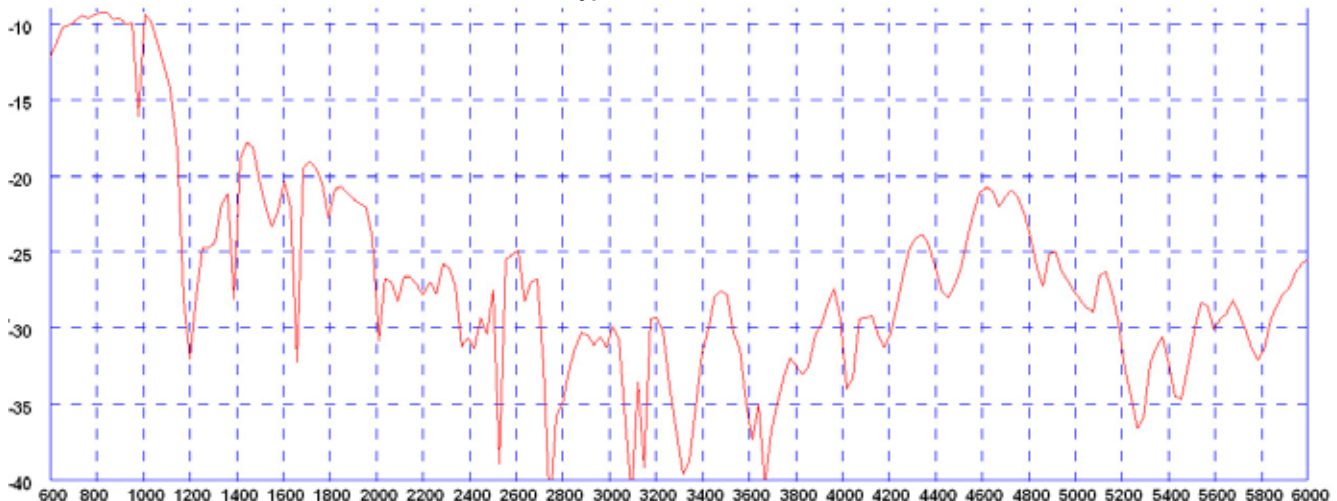
Typical Isolation ****
